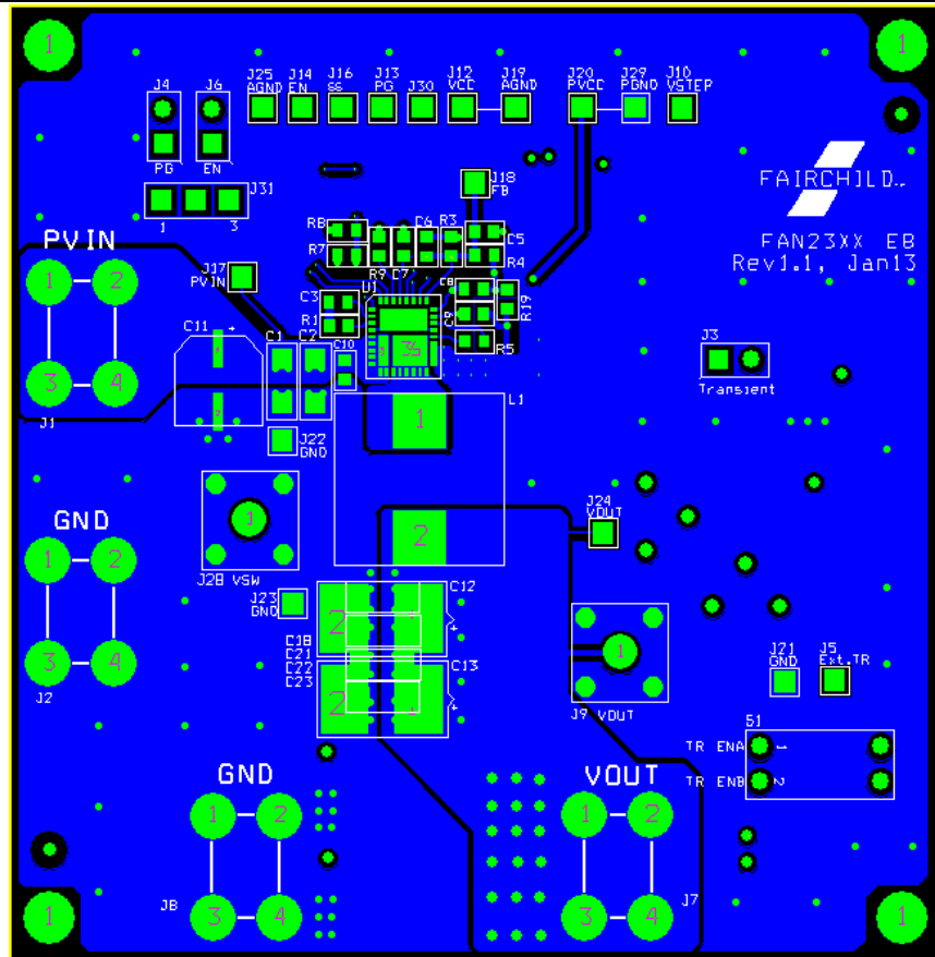
Figure 28. Evaluation Board Top Layer Copper
