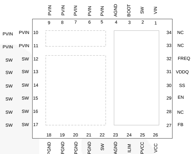
Figure 5. Top View
