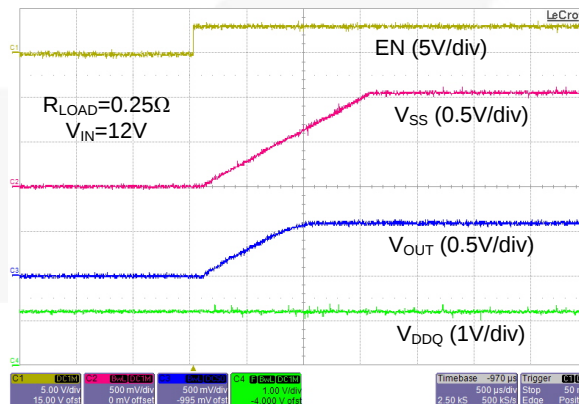
Figure 11. Startup Waveforms Using Soft-Start with 2.4 A Resistive Load
