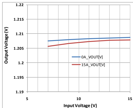
Figure 11. Line Regulation
