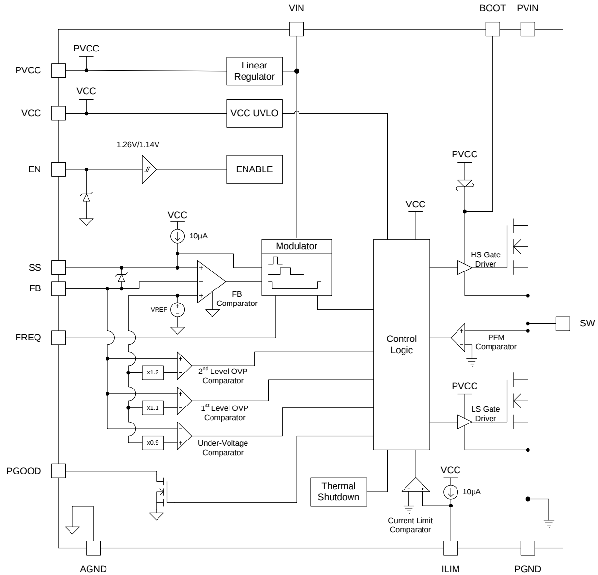
Figure 3. Block Diagram
