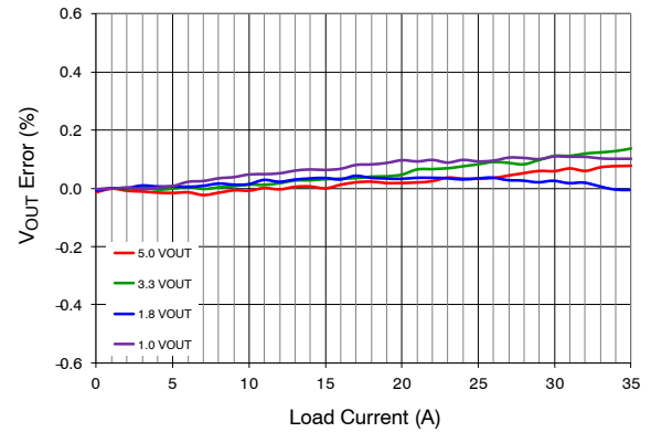
Figure 5. Load Regulation
