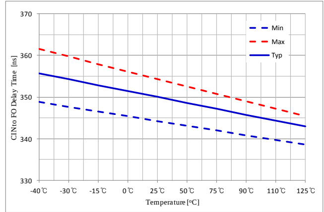
Figure 24. CIN Triggering to FO Delay vs. Temperature
