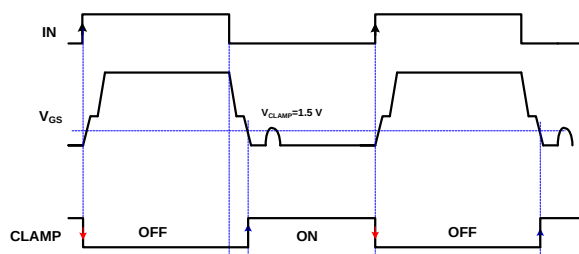
Figure 56. Waveform of Active Miller Clamp
