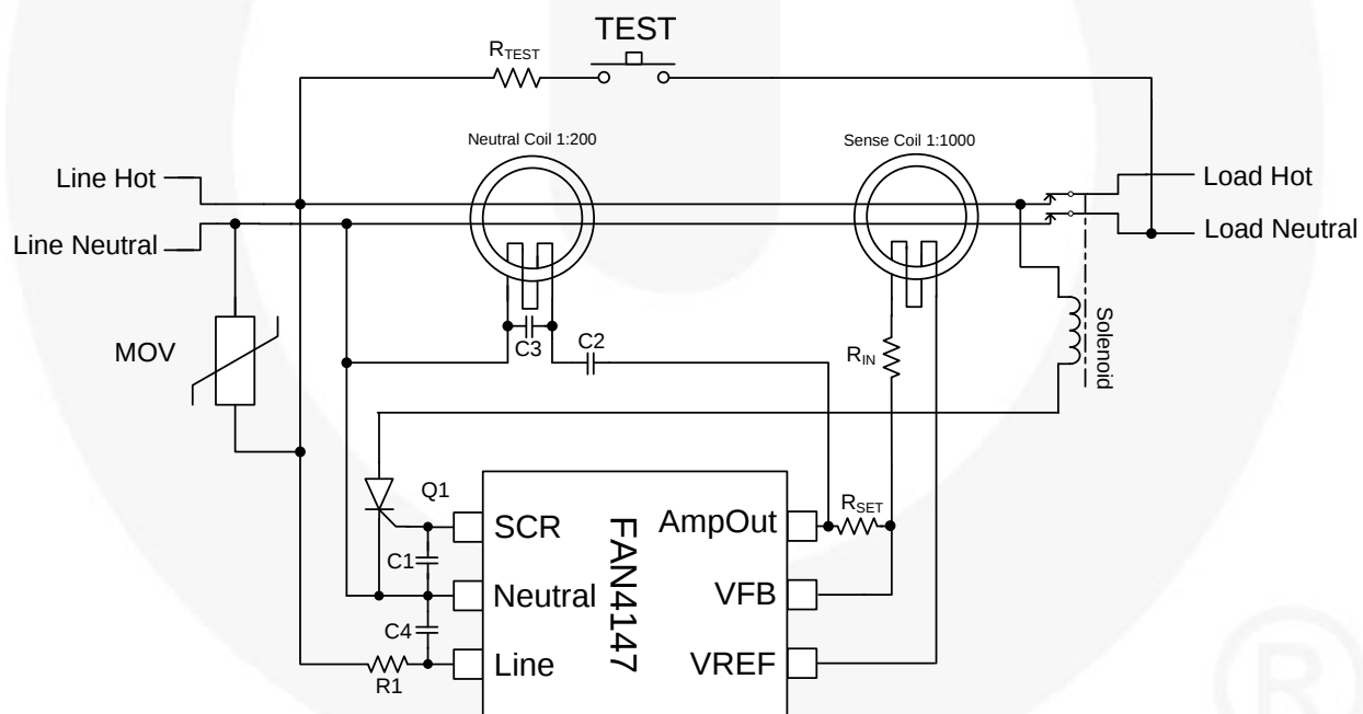
Figure 2. Typical Application (1)
