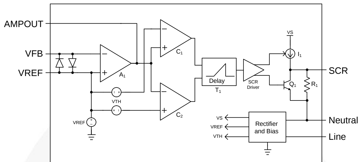
Figure 1. Block Diagram
