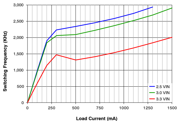
Figure 14. Frequency vs. Load Current and Input Voltage
