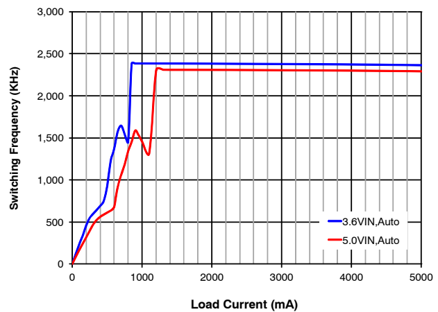
Figure 8. Frequency vs. Load Current
