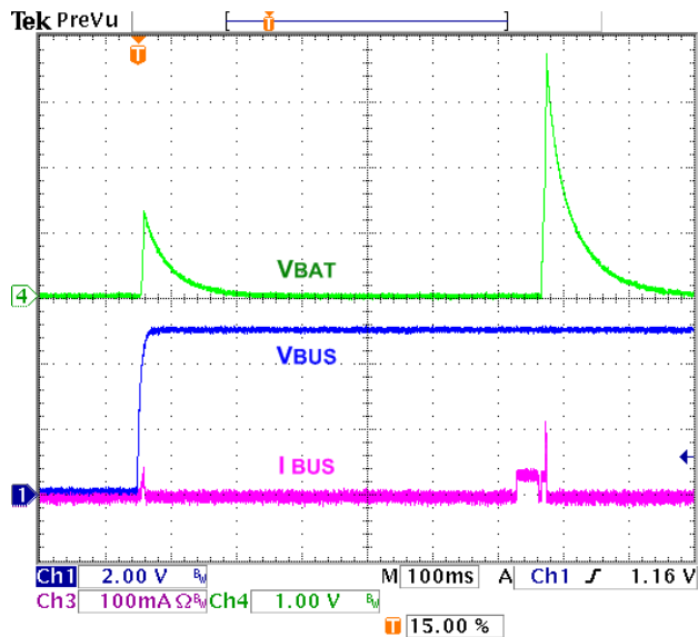
Figure 17. No Battery at V_{\text{BUS}} Power-up; FAN54010, FAN54013
