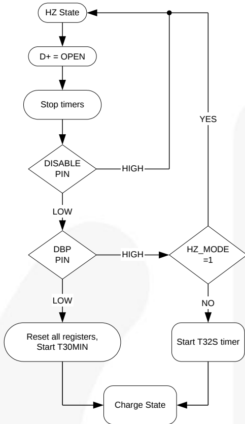
Figure 41. HZ State Flow Chart
