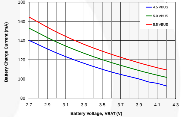
Figure 10. Charge Current vs. Battery Voltage, I_{BUSLIM}=100 mA
