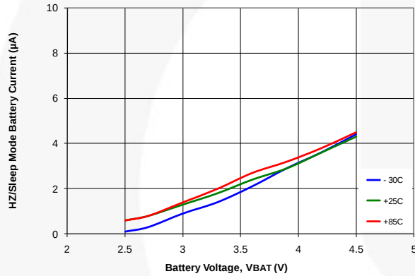
Figure 9. HZ/Sleep Mode Battery Discharge Current, SDA=SCL=1.8 V, DIS=DBP=0
