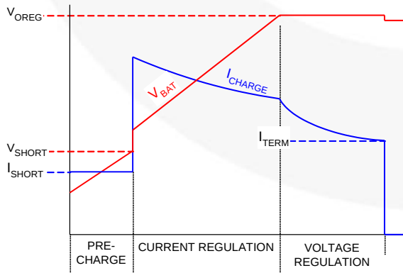
Figure 36. Charge Curve, I_{\text{INLIM}} Limits I_{\text{CHARGE}}
