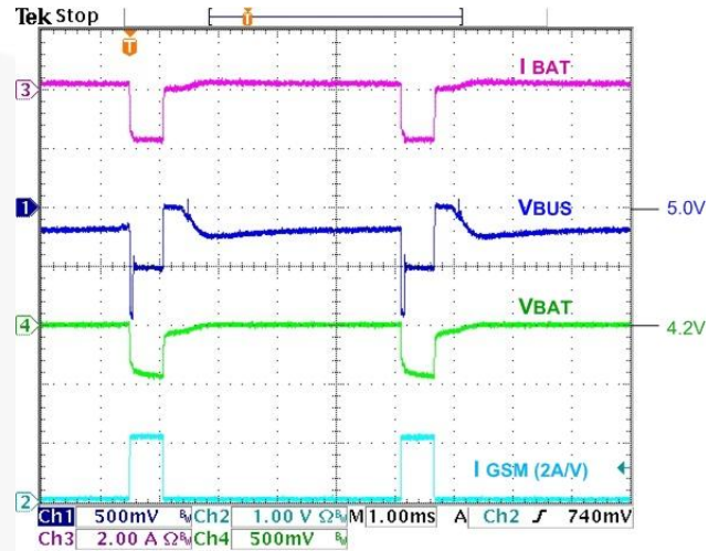
Figure 24. GSM Pulse (2 A Step, t_R/t_F=5\text{ }\mu\text{s} ) Response, 3.9 V BAT , 1 kΩ LDO Load, I_{BUSLIM}=\text{No Limit} , I_{CHRG}=1.0\text{ A} , 500 mA V BUS Source Limited
