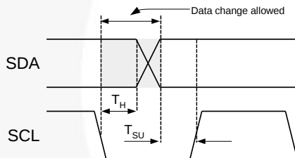
Figure 50. Data Transfer Timing
