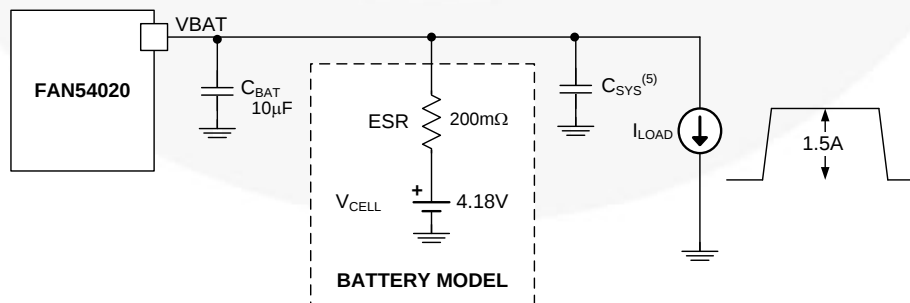
Figure 5. V_{BAT} Overshoot Test Conditions
