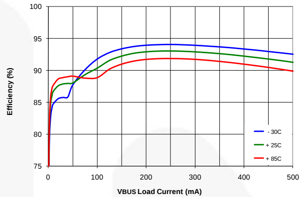
Figure 26. Efficiency vs. Load Current Over-Temperature Range, 3.6 V_{BAT}
