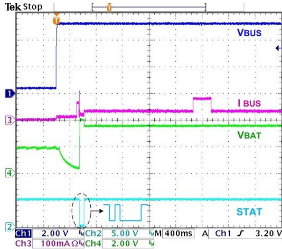
Figure 19. Charger Startup at V_{BUS} Plug-In, No Battery, ILIM=DBP=0 , 300\text{ }\Omega LDO Load
