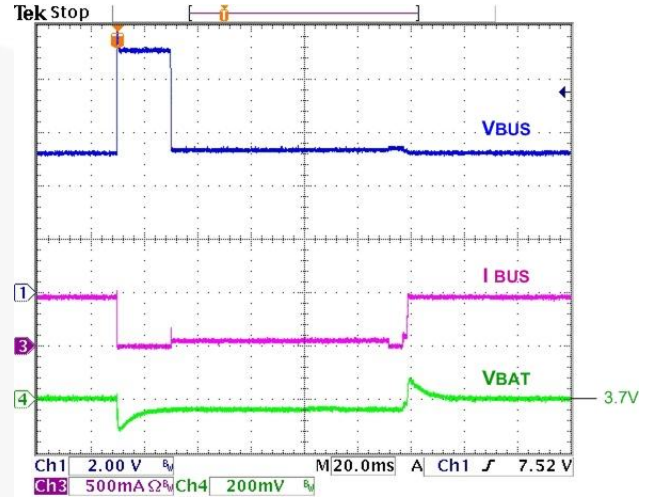
Figure 20. V_{BUS} OVP Response while Charging, 5-9-5\text{ V}_{BUS} , 3.7\text{ V}_{BAT} , I_{BUSLIM}=500\text{ mA} , I_{CHRG}=1.0\text{ A}
