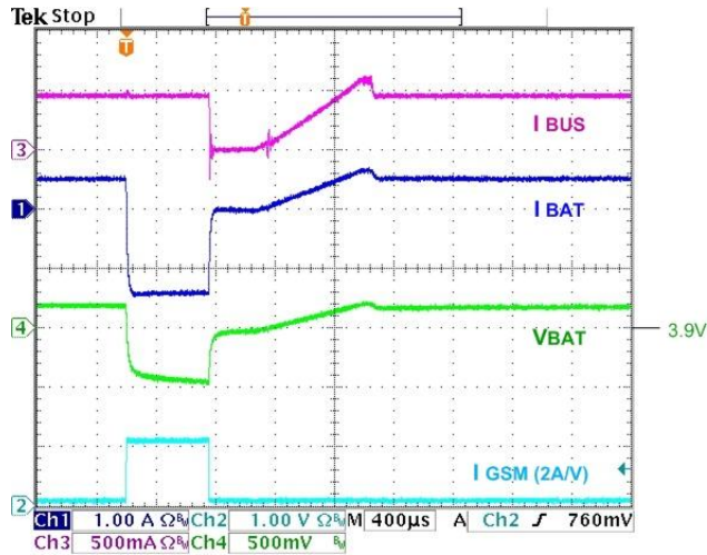
Figure 23. GSM Pulse (2 A Step, t_R/t_F=5\text{ }\mu\text{s} ) Response, 3.9 V BAT , 1 kΩ LDO Load, I_{BUSLIM}=500\text{ mA} , I_{CHRG}=1.0\text{ A}
