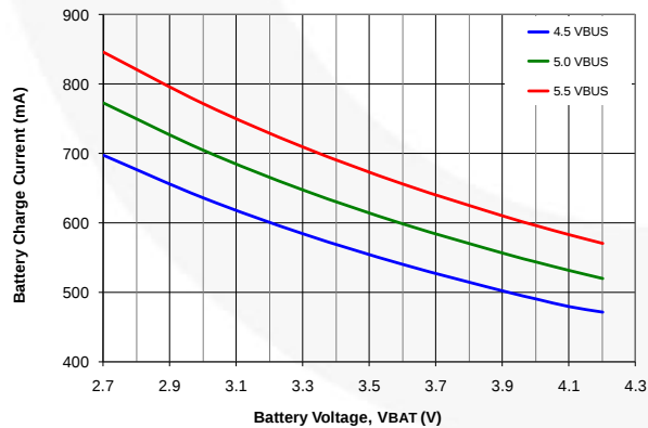
Figure 11. Charge Current vs. Battery Voltage, I_{BUSLIM}=500 mA
