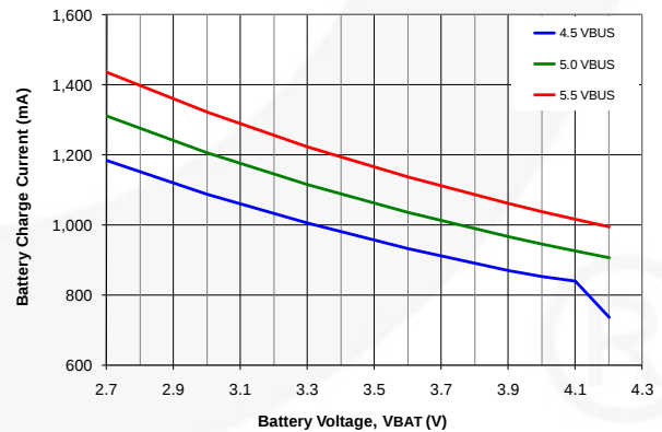
Figure 12. Charge Current vs. Battery Voltage, I_{BUSLIM}=900 mA
