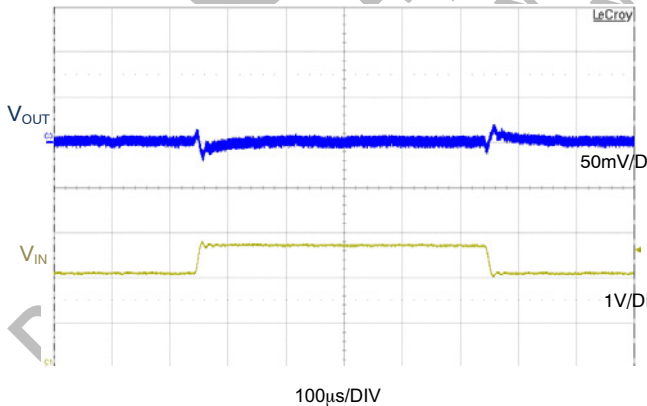
Figure 21. Line Transient, V_{IN} = 3.6\text{ V} to 4.2\text{ V} , V_{OUT} = 1.0\text{ V} , 6.8\ \Omega Load, 10\ \mu\text{s} Edge
