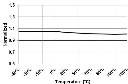
Figure 8. Operating Current Over 5 V ( I_{IN-OP-9V,12V} ) vs. Temperature
