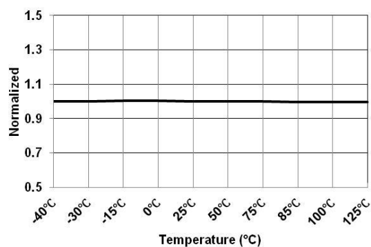
Figure 25. V_{IN} UVP Disable Voltage at 9 V ( V_{IN-UVF-H-9V} ) vs. Temperature
