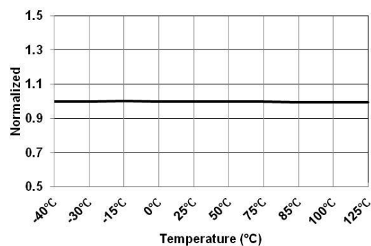
Figure 26. V_{IN} UVP Enable Voltage at 12 V ( V_{IN-UVF-L-12V} ) vs. Temperature
