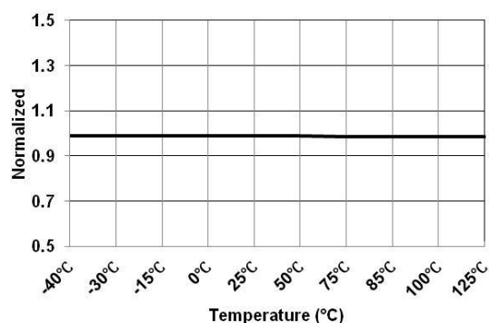
Figure 27. V_{IN} UVP Disable Voltage at 12 V ( V_{IN-UVF-H-12V} ) vs. Temperature
