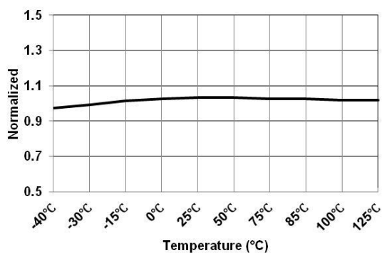
Figure 7. Operating Current Under 5 V ( I_{IN-OP-5V} ) vs. Temperature
