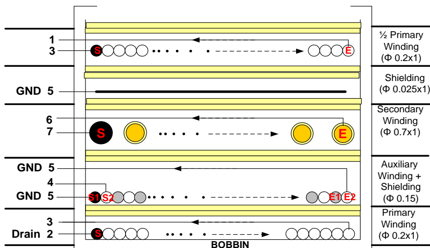
Figure 42. Transformer Diagram
