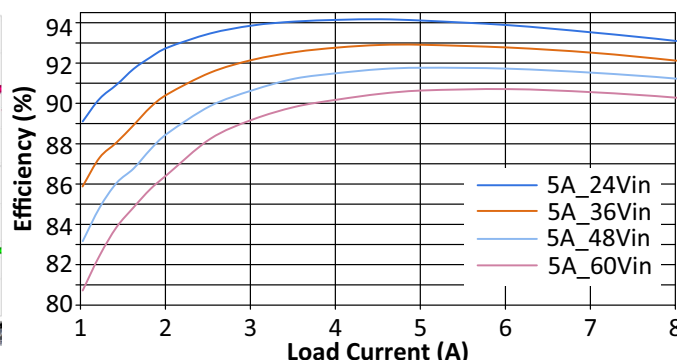
Figure 37. System Efficiency
