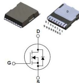
H-PSOF8L 11.68x9.80 CASE 100CU
