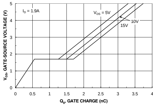
Figure 7. Gate-Charge Characteristics.
