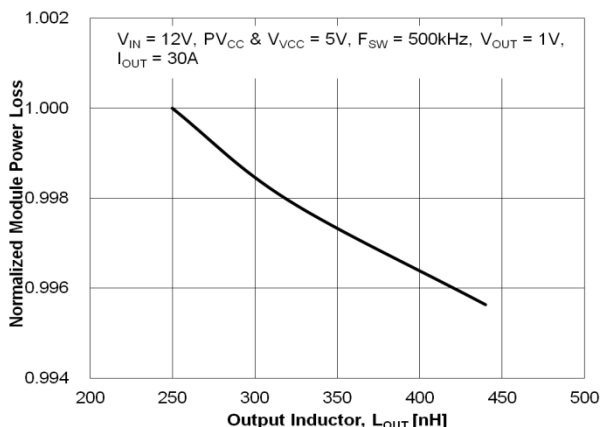
Figure 12. Power Loss vs. Output Inductor
