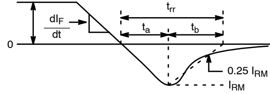
Figure 2. t_{rr} Waveform and Definitions
