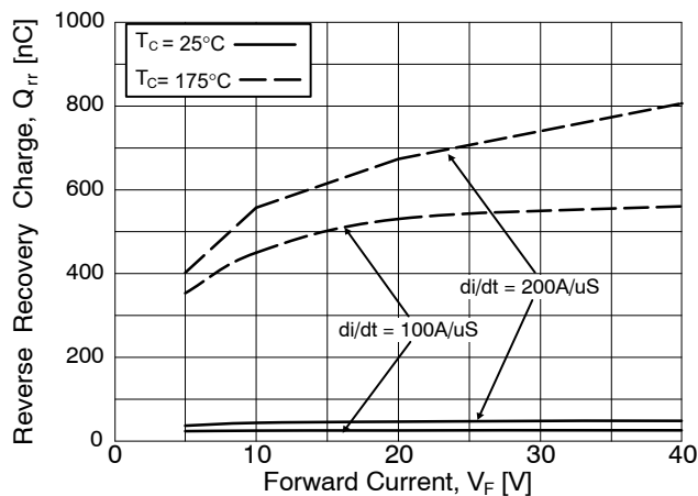
Figure 18. Stored Charge
