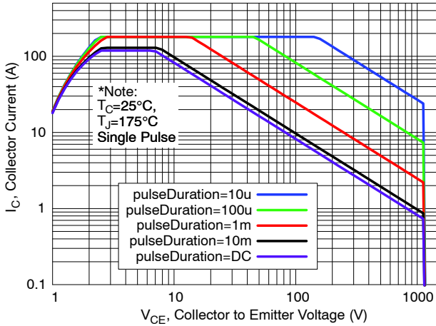
Figure 9. SOA Characteristics
