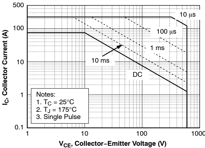
Figure 17. SOA Characteristics
