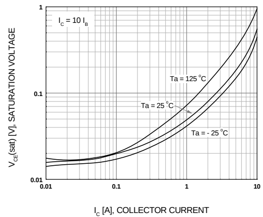
Figure 4. Collector-Emmitter Saturation Voltage
