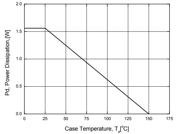
Figure 10. Power Derating
