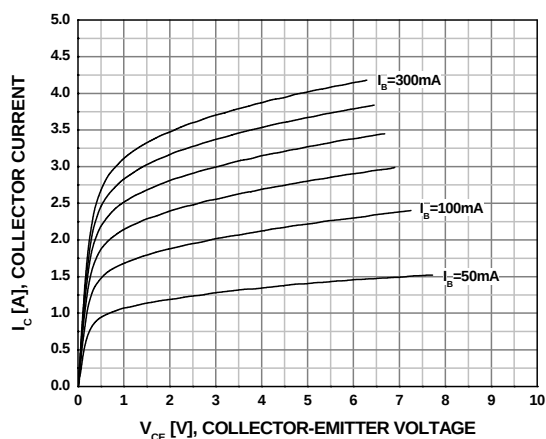
Figure 1. Static Characteristic
