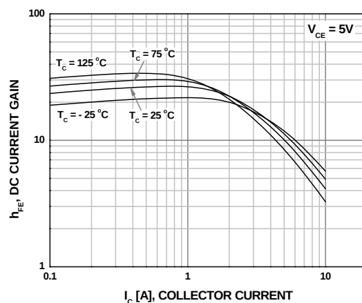
Figure 2. DC Current Gain (H1 Grade)
