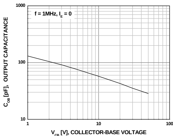
Figure 6. Output Capacitance
