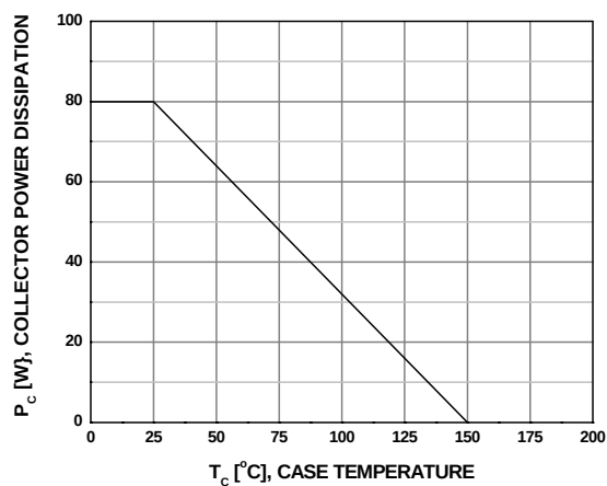
Figure 7. Power Derating
