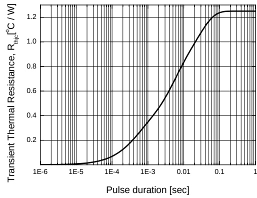
Figure 7. Thermal Resistance
