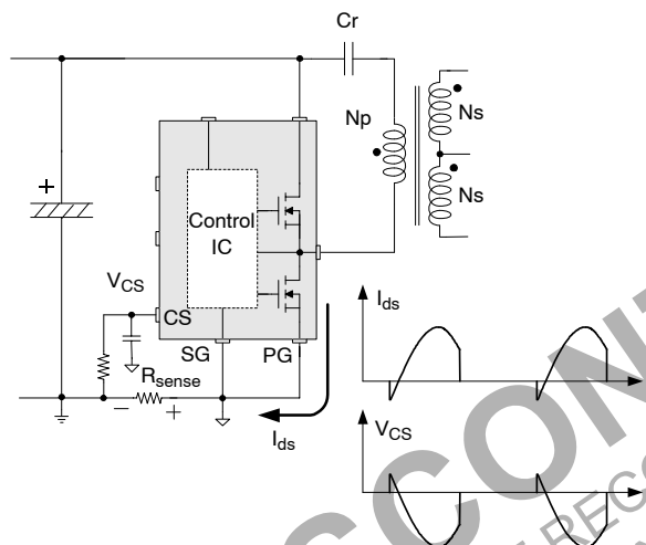
Figure 23. Half-Wave Sensing
