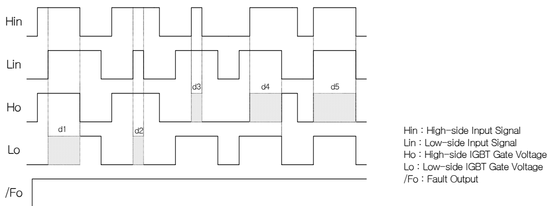
Figure 11. Short-Circuit Protection
