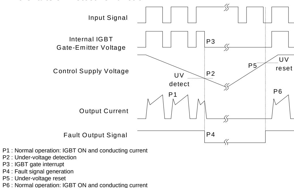
Figure 7. Under-Voltage Protection
