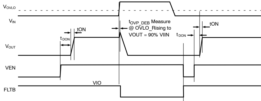
Figure 7. OVP Operation
