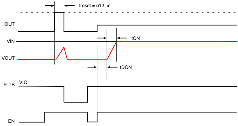
Figure 5. Inrush Current Limit and SCP Operation (Latch-Off)
