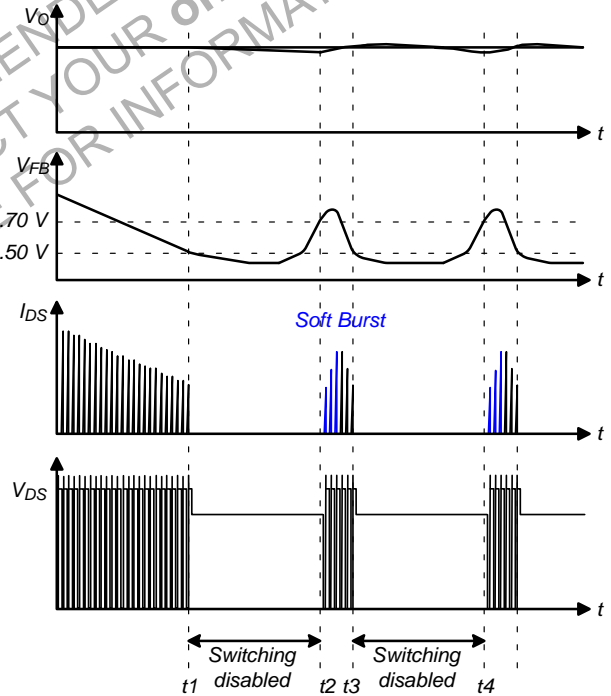
Figure 23. Burst–Mode Operation
