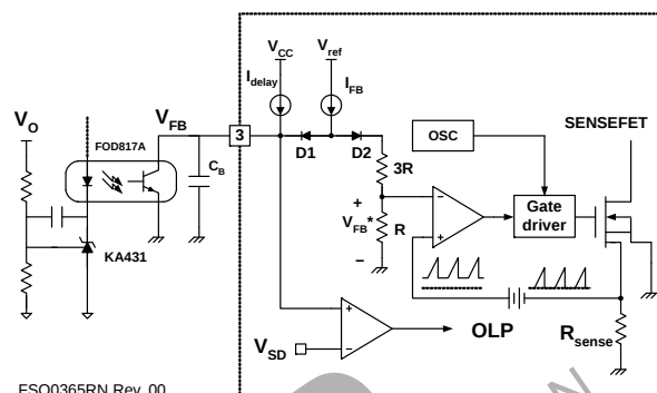
Figure 21. Pulse-Width-Modulation Circuit
