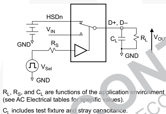
Figure 7. AC Test Circuit Load
