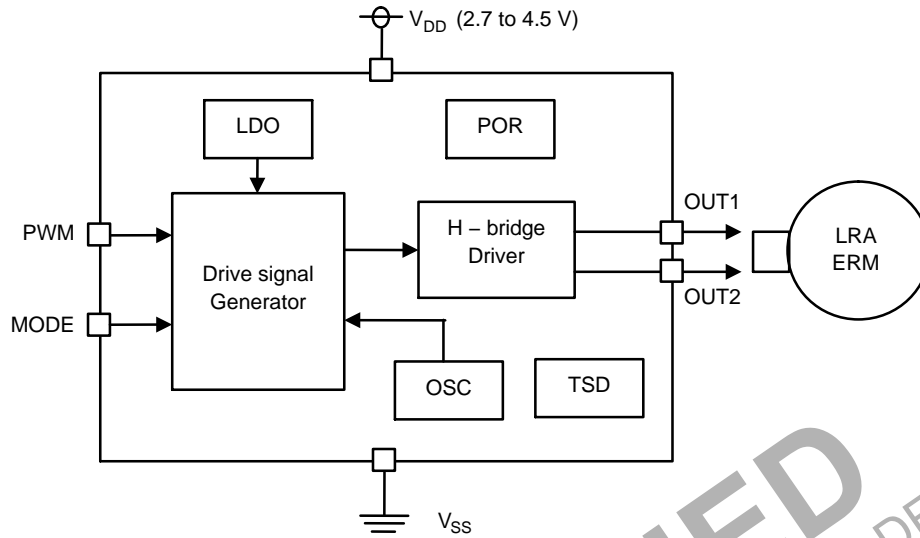
Figure 1. Block Diagram
