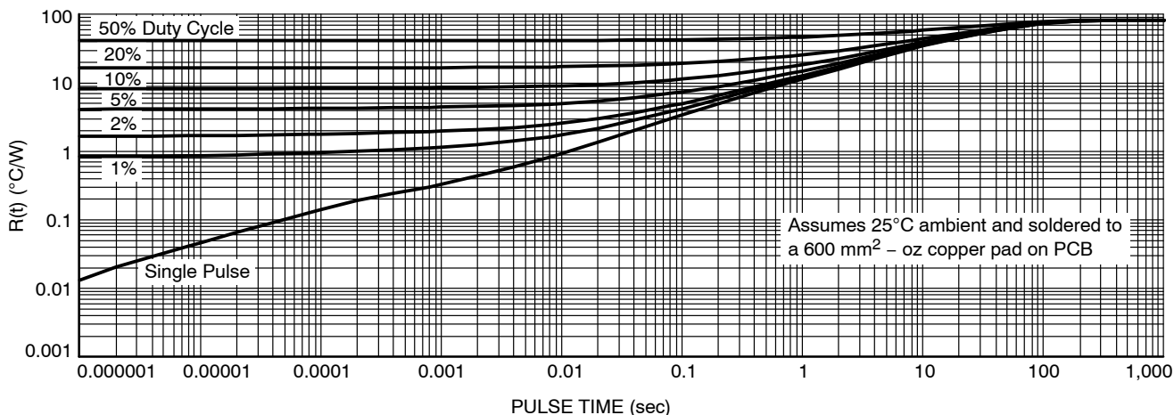
Figure 8. Thermal Response
