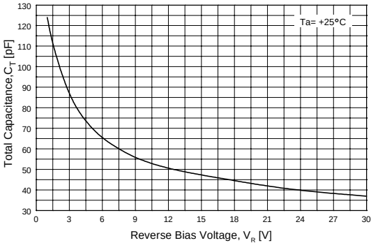
Figure 3. Total Capacitance
