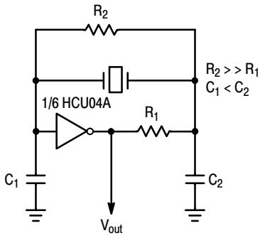
Figure 5. Crystal Oscillator
