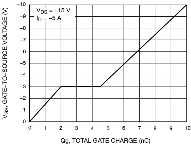
Figure 10. V_{GS} - Q_g
