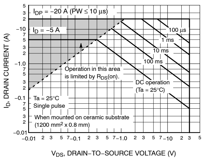
Figure 11. SOA
