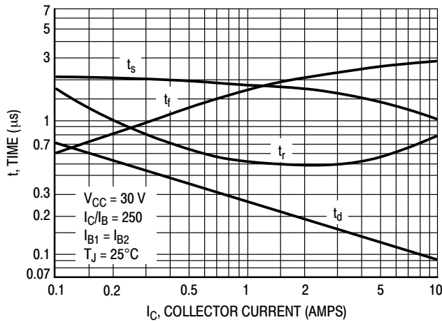
Figure 3. Typical Switching Times
