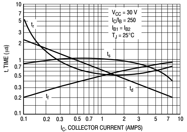
Figure 3. Typical Switching Times
