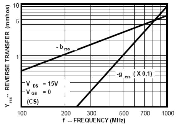
Figure 14. Reverse Transadmittance
