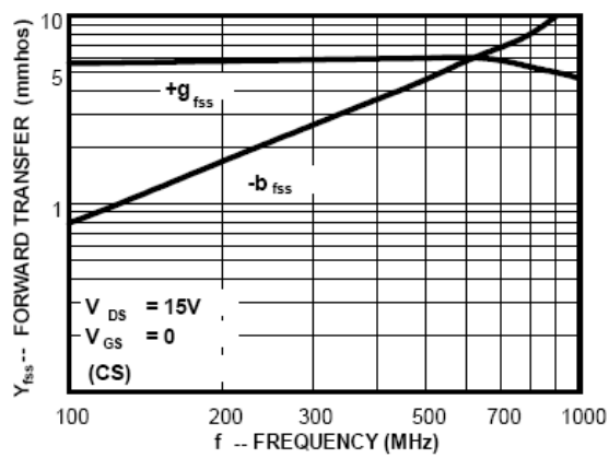
Figure 13. Forward Transadmittance
