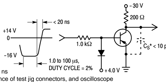
Figure 2. Turn–Off Time
