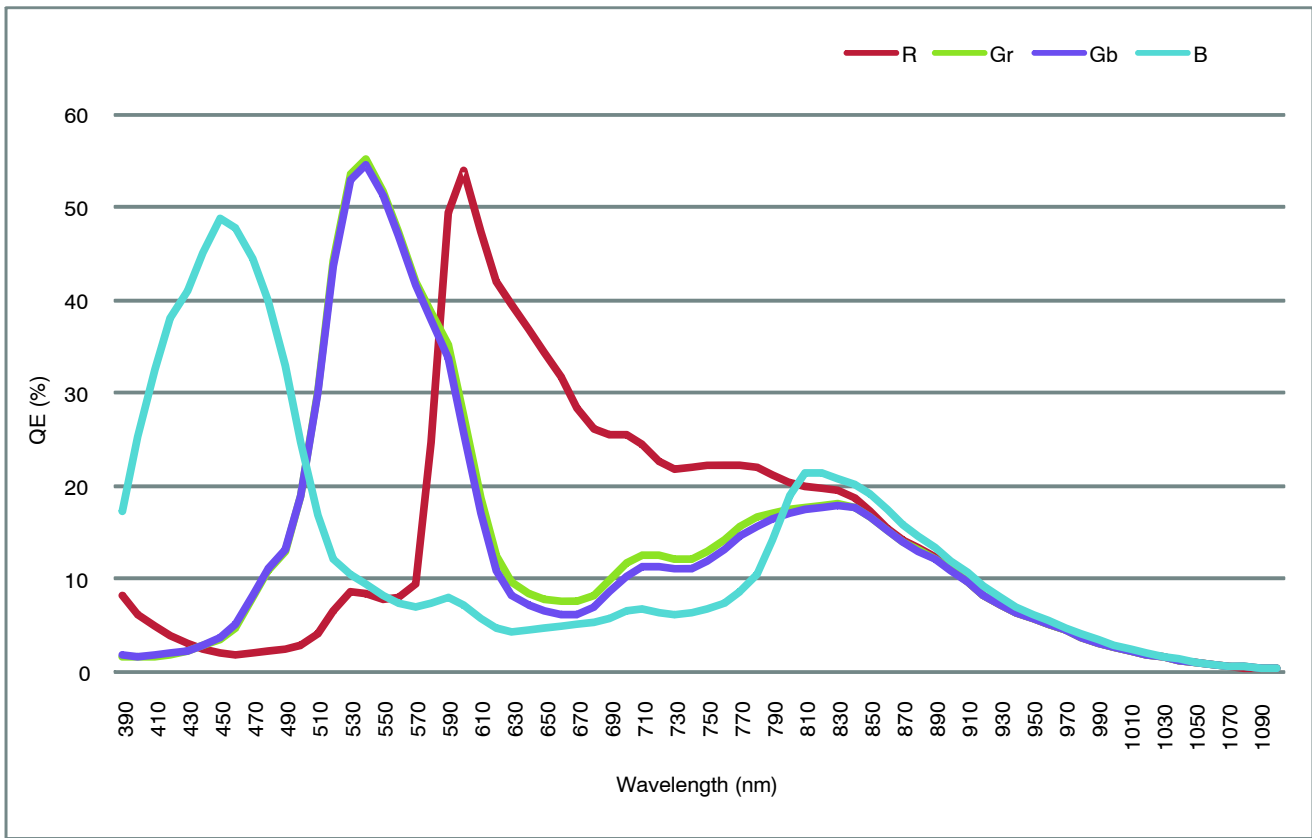
Figure 29. Quantum Efficiency
