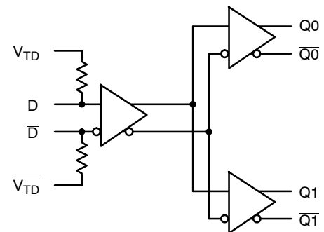
Figure 1. Logic Diagram
