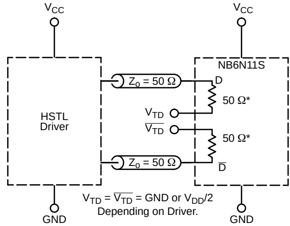
Figure 14. HSTL Interface
