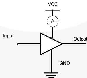
Figure 4. I CCD Test Circuit
