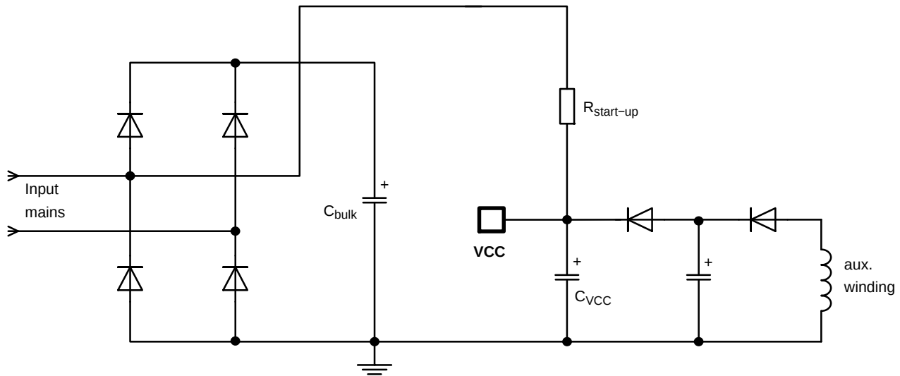
Figure 38. The Startup Resistor can be Connected to the Input Mains for further Power Dissipation Reduction
