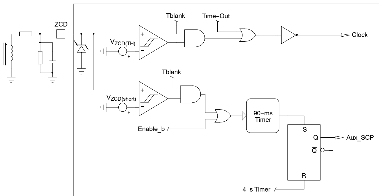
Figure 65. ZCD Block Schematic
