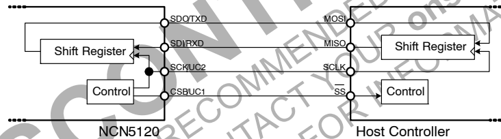
Figure 27. SPI Master
