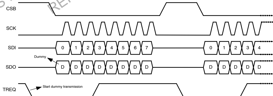
Figure 28. Transmission Request
