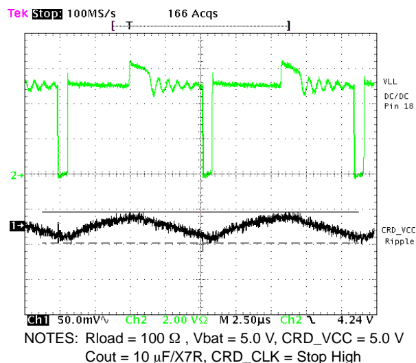
Figure 23. CRD_VCC Voltage Ripple
