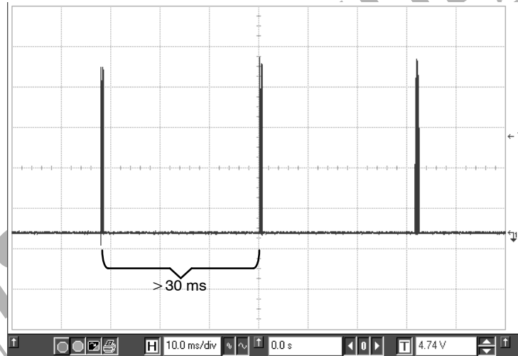
Figure 18. The Burst Frequency becomes So Low that it is Difficult to Keep an Adequate Level on the Auxiliary V_{CC}
