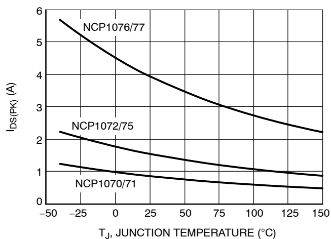
Figure 22. Drain Current Peak during Transformer Saturation vs. Junction Temperature
